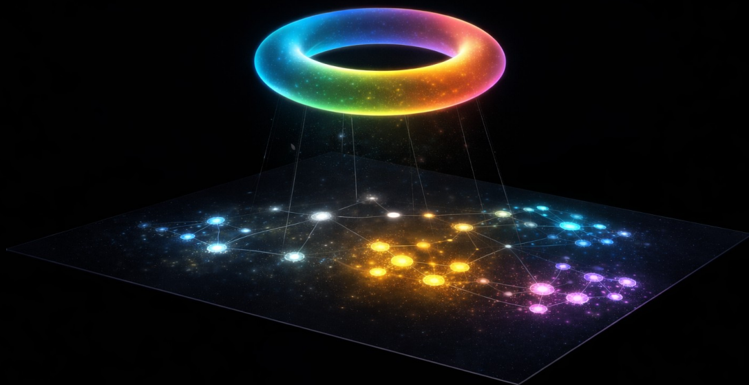
Figure 12: Conceptual depiction of emergent spacetime interpreted as a projection of structured causal relationships within a Miranova Matrix frame.
