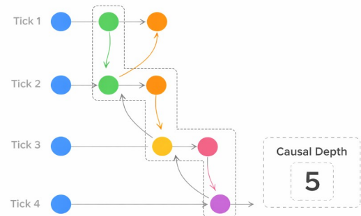
Figure 3: Causal depth as the longest chain of tick-ordered dependencies.
